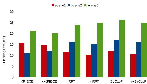
Fig. 15 Histogram of the average planning time. Scene1, scene2 and scene3 correspond to the scenes illustrated in Fig. 9.
