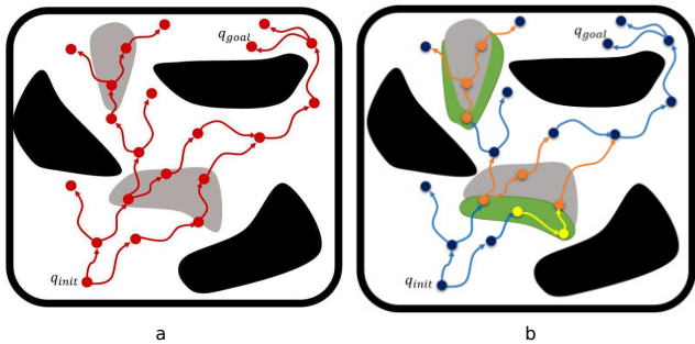
Fig. 7 Sample and propagation using: (a) the simple physics-based motion planner; (b) \kappa -PMP. The control sampling range is selected based on the dynamics properties of the target object and the manipulation region. Blue samples represent the lower values of control range, whereas orange samples represent the higher values. Yellow samples represents the decrease in forces during the transition between free and contact motions.
