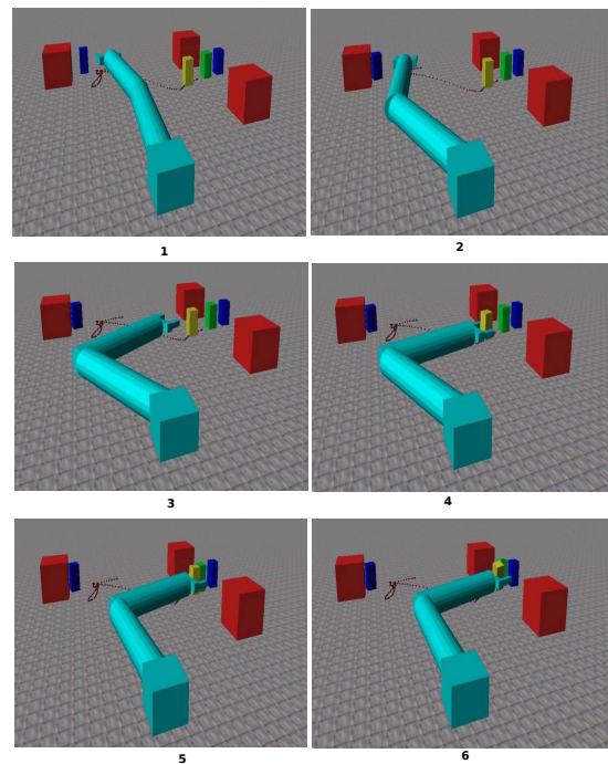
Fig. 17 Execution of the computed motion plan by the simple physics-based motion planner. It can be observed that the task fails because the manipulatable yellow object ends at the gripper, thus preventing the manipulator to grasp the target green object.
