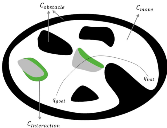
Fig. 2 Configuration space: C_{obs} shown in black (collisions with fixed obstacles) and gray (collision with manipulatable obstacles), C_{interaction} in green and C_{move} in white.
