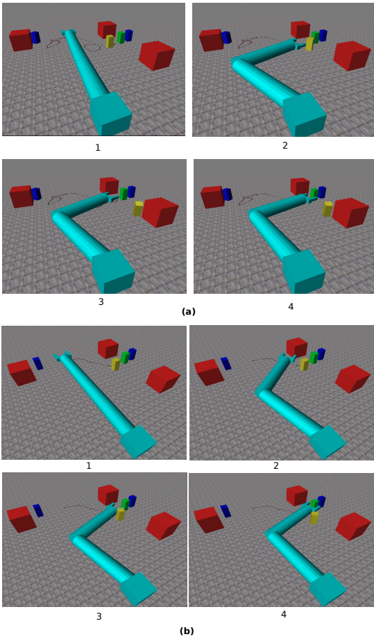
Fig. 18 Snapshots of the dynamic interactions between the robot and the yellow object corresponding to the simple physics-based motion planning (a) and to the \kappa -PMP planner (b), respectively. Videos: https://sir.upc.edu/projects/kautham/videos/k-PMP2.mp4
